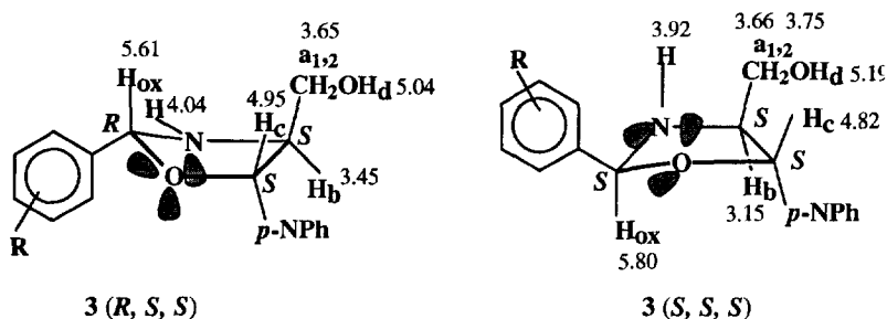
Scheme 6 (only \delta -values for the 3I epimers are depicted)
