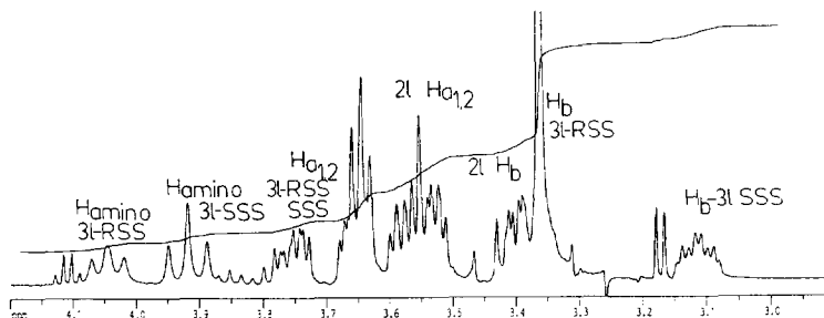
Figure 7: ^1\text{H} -NMR spectrum (detail) of the Schiff base 2l and its tautomers (epimeric oxazolidines 3l ) after 350h
