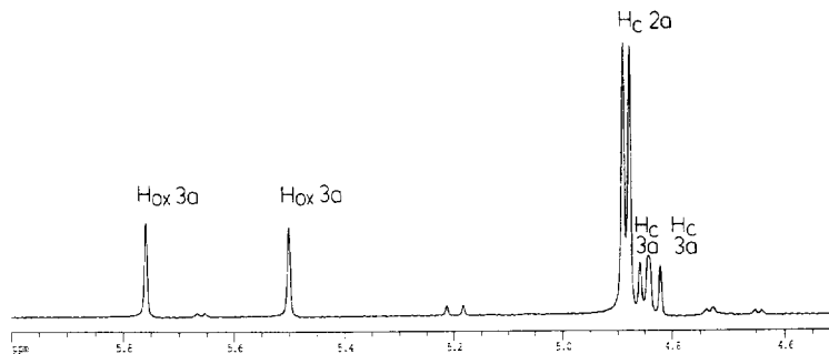
Figure 4: ^1\text{H} -NMR-spectrum (detail) including the reference protons of the compound 2a and its tautomers 3a , after 100h ( \text{DMSO-d}_6 + \text{D}_2\text{O} )
